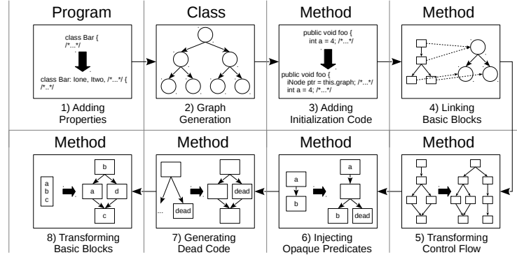
Fig. 1. The eight steps of the obfuscation process. On the top, it is noted which entity is targeted by the current obfuscation step.
